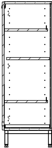
SECTION C-C
